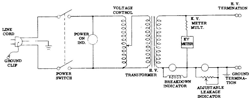
HYPOT JUNIOR SIMPLIFIED SCHEMATIC
