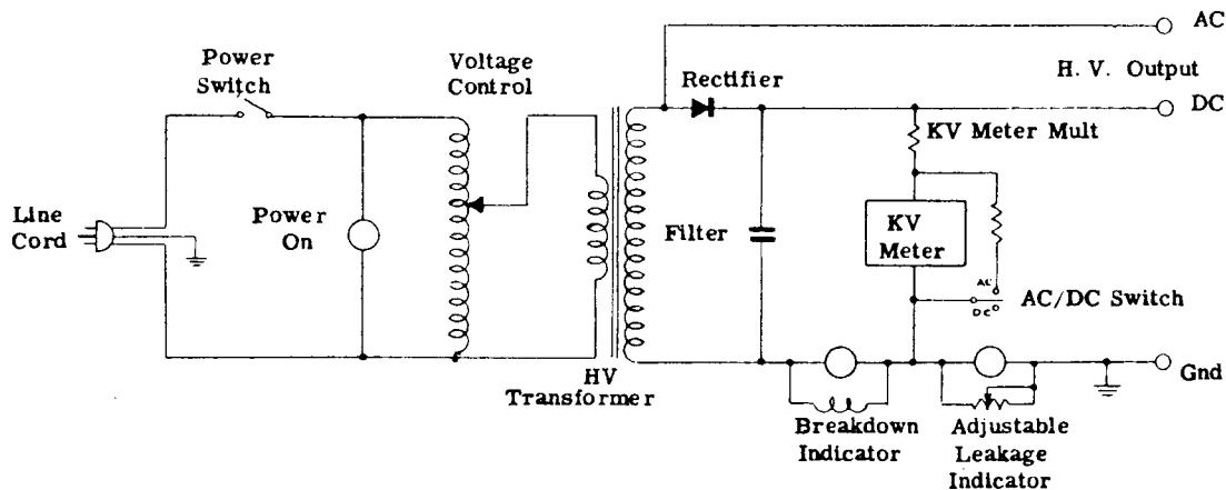
DC HYPOT ® JUNIOR SIMPLIFIED SCHEMATIC
