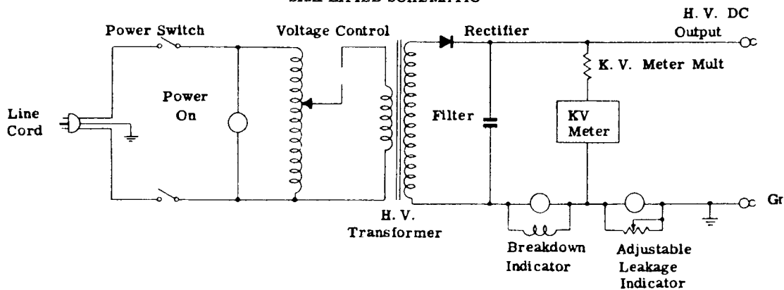
DC HYPOT ® JUNIOR SIMPLIFIED SCHEMATIC
